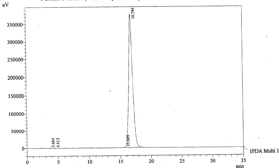
Chromatogram 8-Bromo-6-chloro-2',5'-dimethoxyflavone D:\promonence\Data\2013\AUG-2013\300813M.lcd
